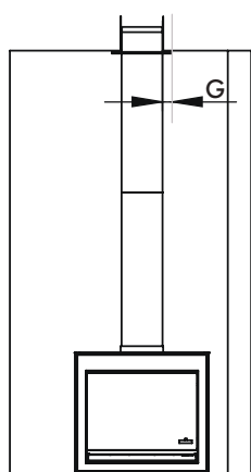
Firebox
