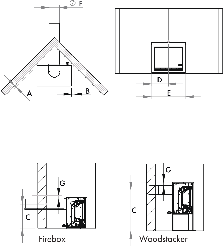
CORNER CLEARANCE
