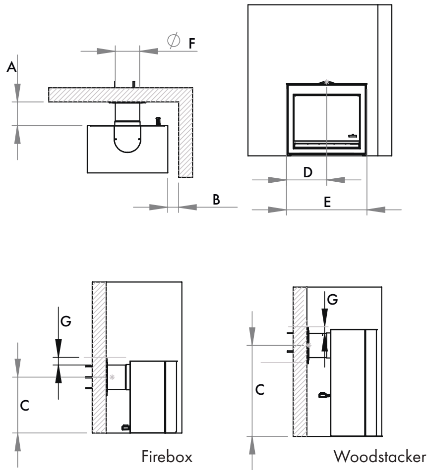
WALL CLEARANCE
