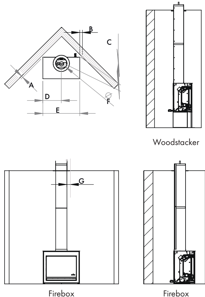
CORNER CLEARANCE
