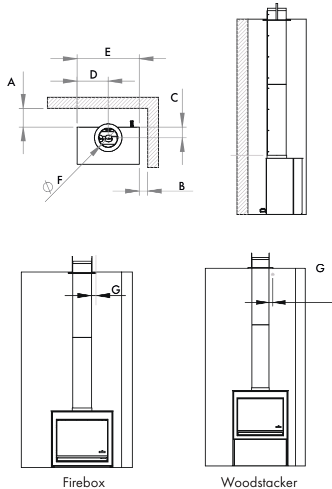
WALL CLEARANCE
