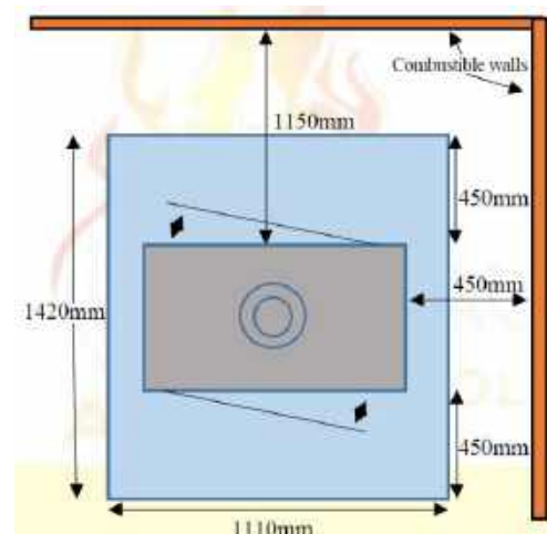
Figure No.8 - Safety distances for Verona 800/801
